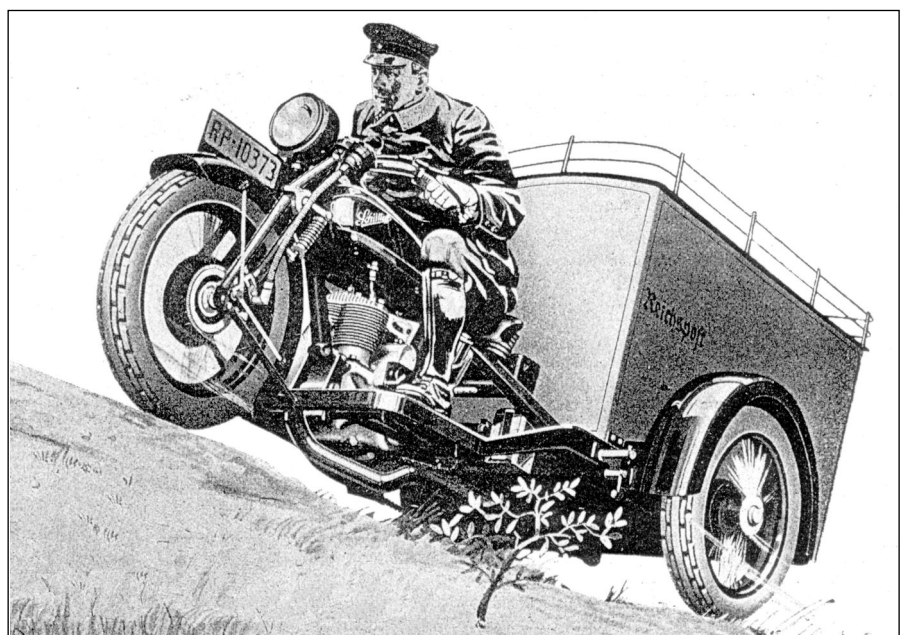
Schüttoff-Transport-Dreirad 1929 1
